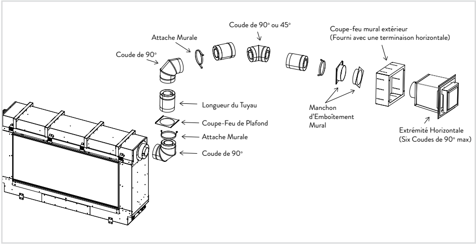
Horizontal termination example layout
