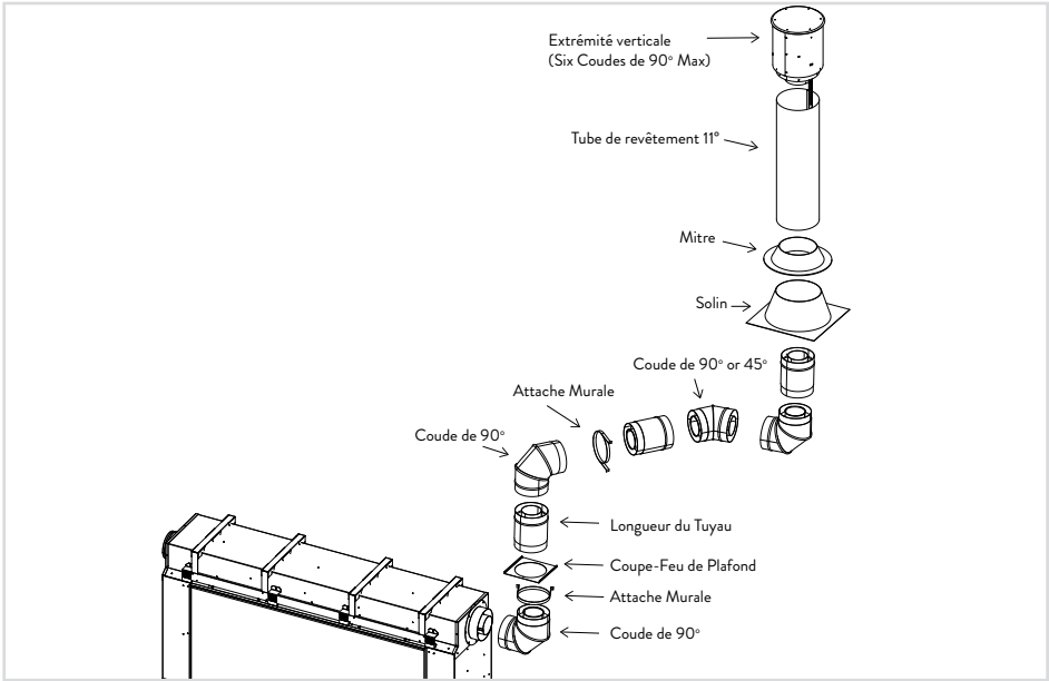
Vertical termination example layout
