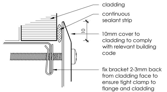
Fixing Detail scale 1:1
