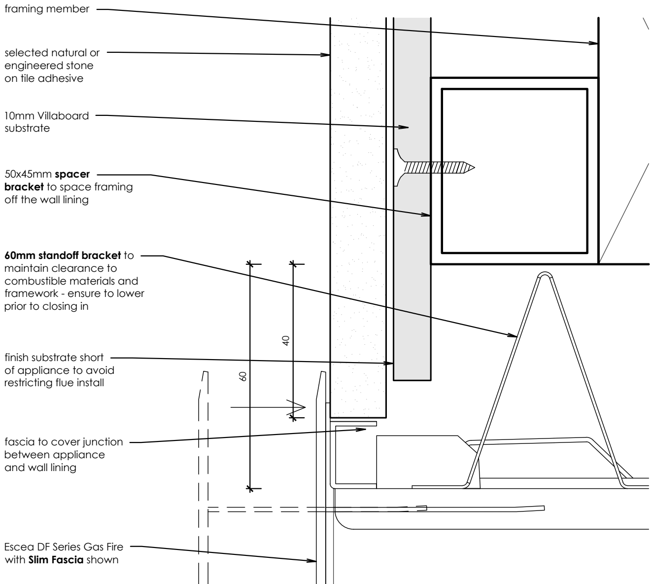
Head Detail
