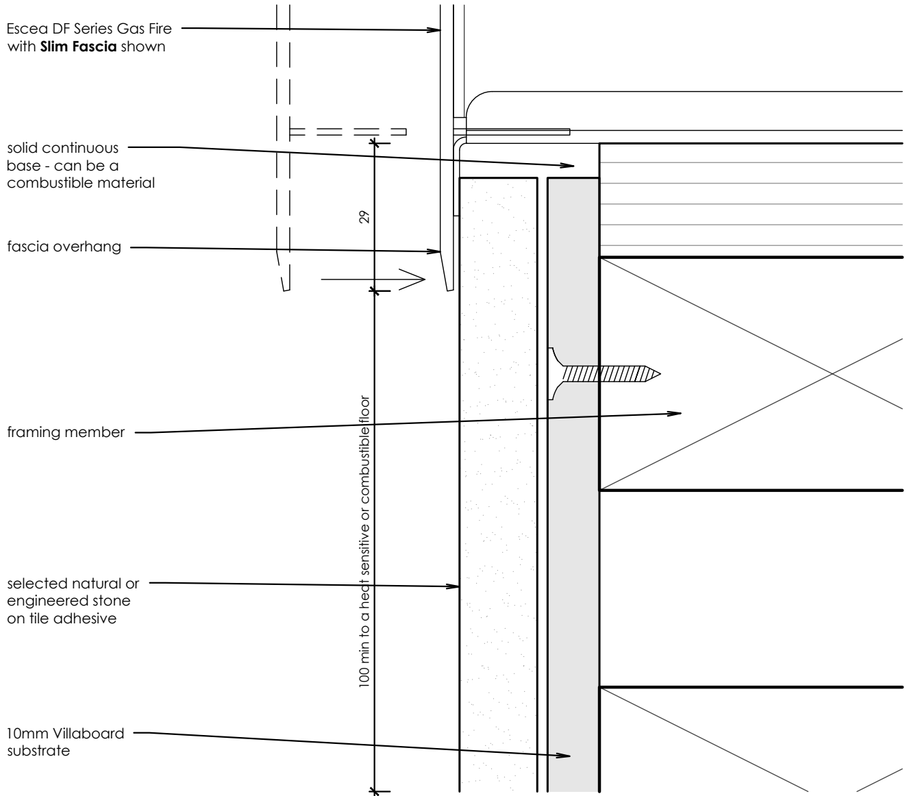
Base Detail
