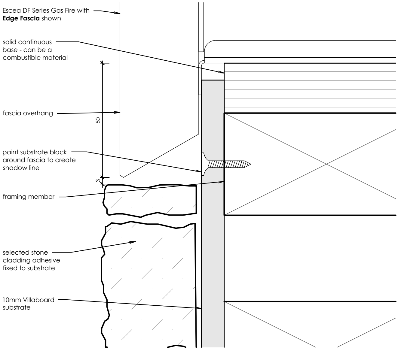
Base Detail
