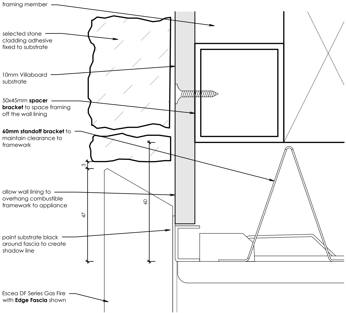
Head Detail
