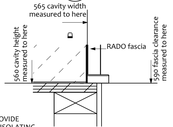
6 RECESSED BASE Scale: 1:5
