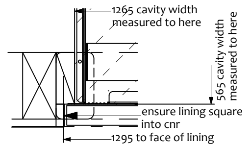
5 RECESSED JAMB Scale: 1:5
