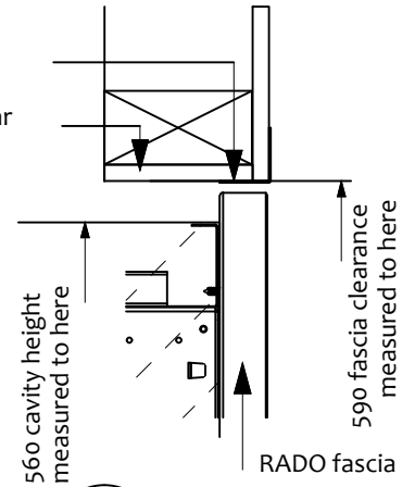
4 RECESSED HEAD Scale: 1:5
