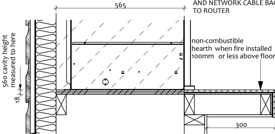
3 FLOOR DETAIL Scale: 1:10
