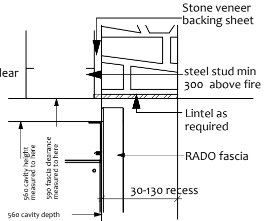
4 RECESSED HEAD Scale: 1:5
