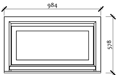
6 RECESSED BASE Scale: 1:5
