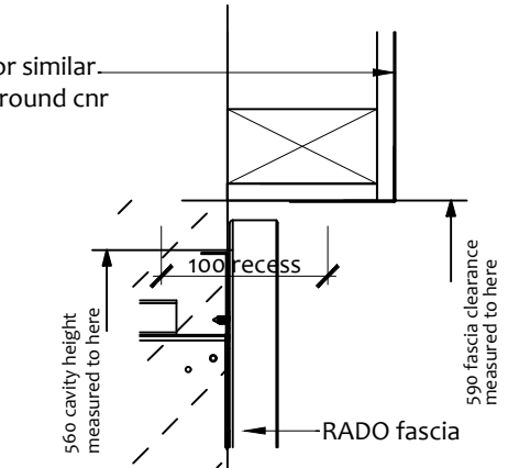
4 RECESSED HEAD Scale: 1:5
