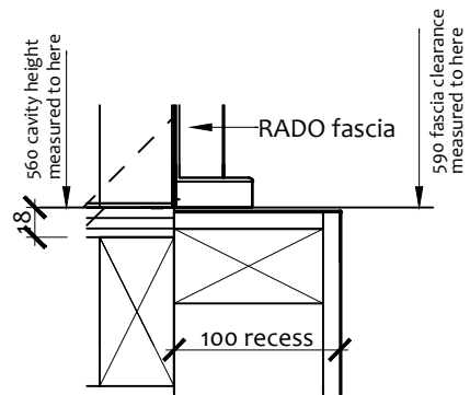
6 RECESSED BASE Scale: 1:5
