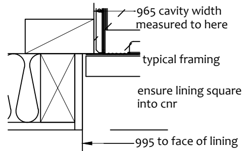
5 RECESSED JAMB Scale: 1:5
