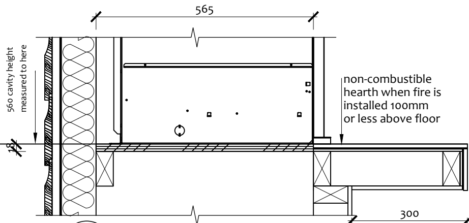
3 FLOOR DETAIL Scale: 1:10
