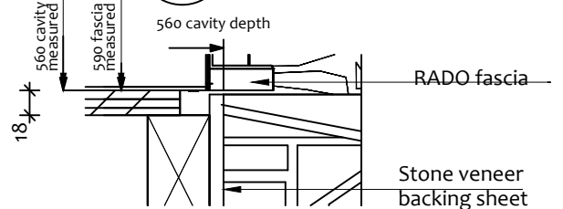
6 RECESSED BASE Scale: 1:5
