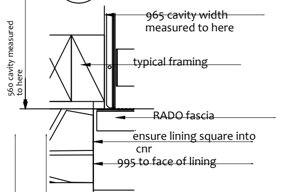
5 RECESSED JAMB Scale: 1:5
