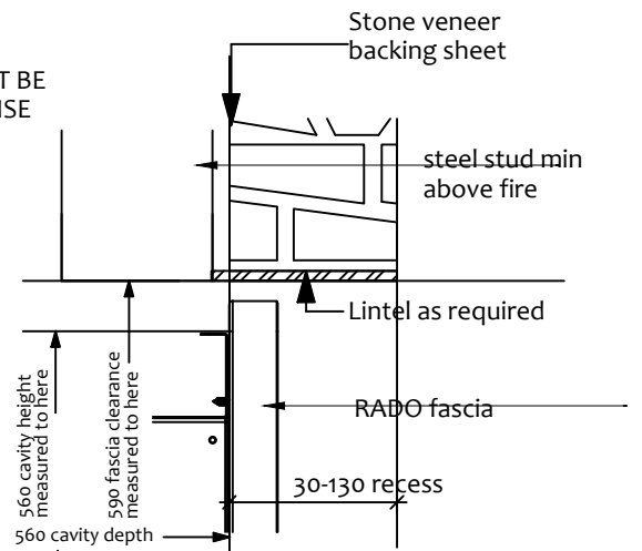
4 RECESSED HEAD Scale: 1:5
