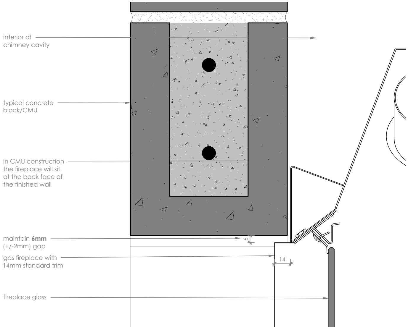
Concrete Detail
