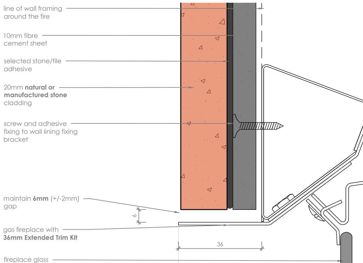
Stone Detail
