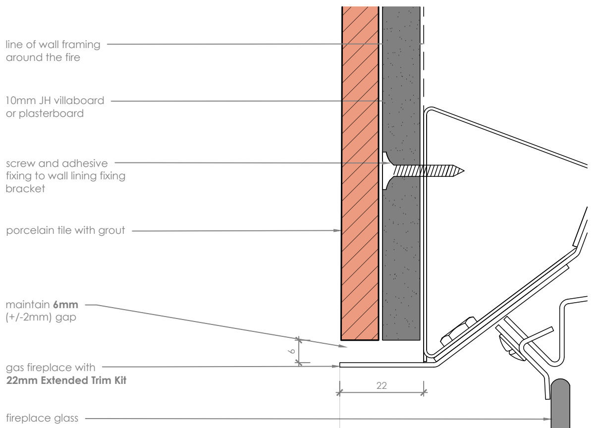
Tile Detail
