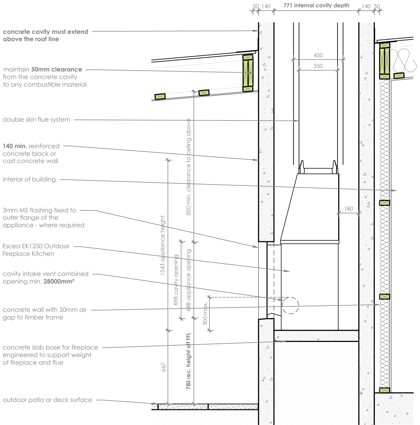
Section - Side
