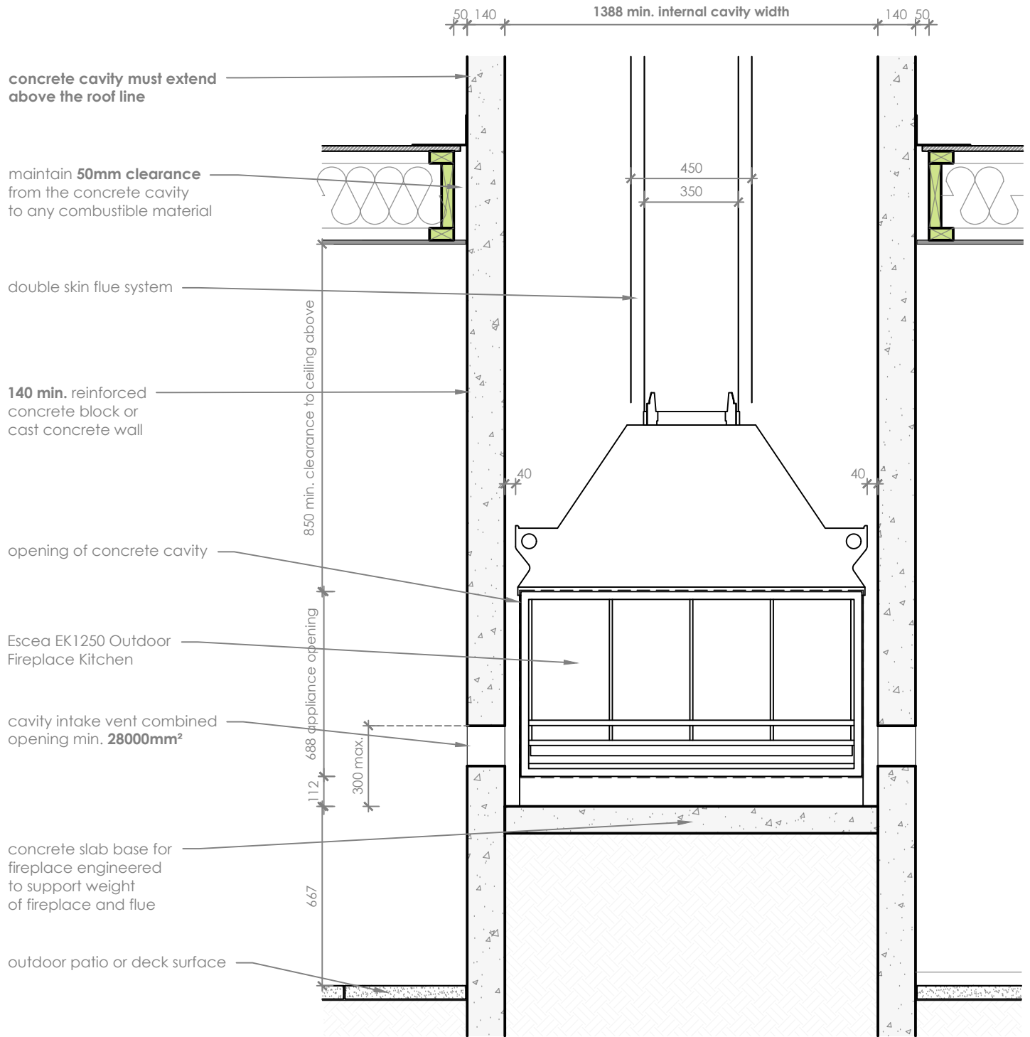
Section - Front
