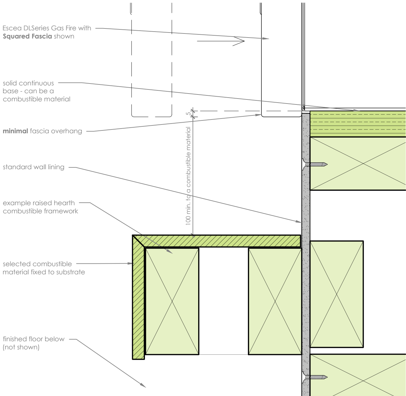
Squared Fascia Detail
