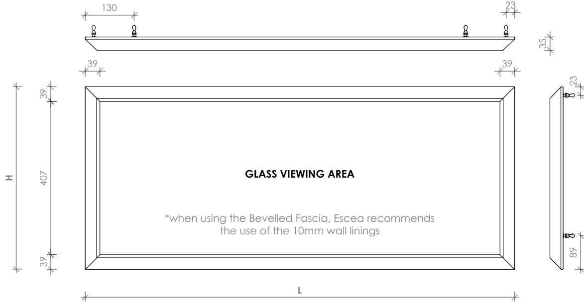
Bevelled Fascia scale 1:10
