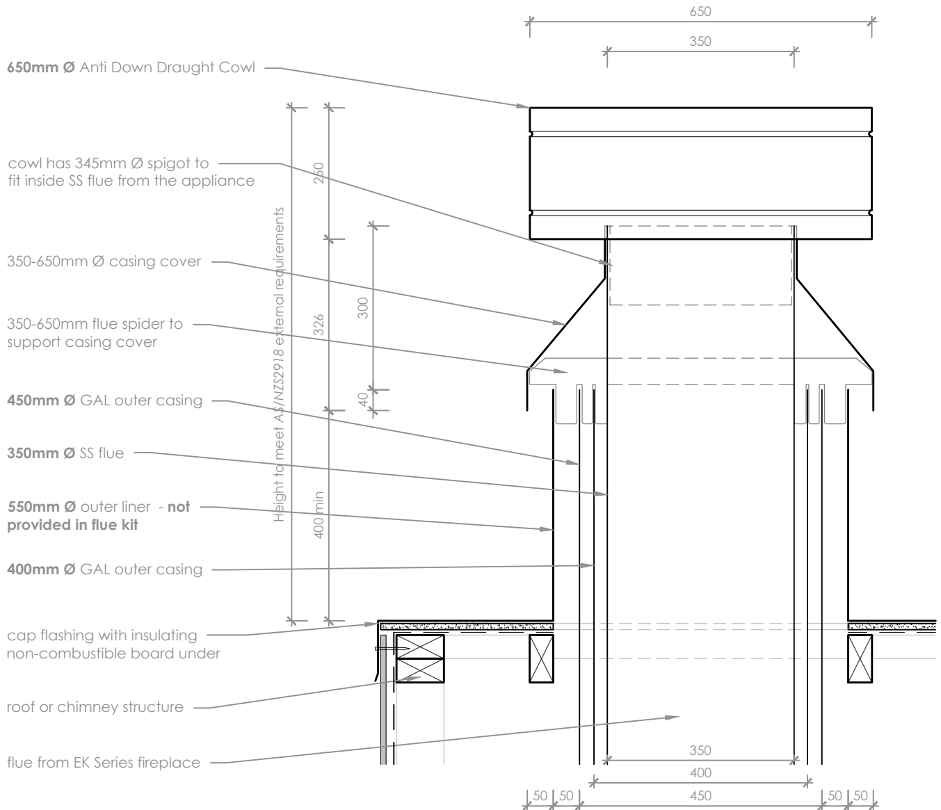
Chimney Chase Detail
