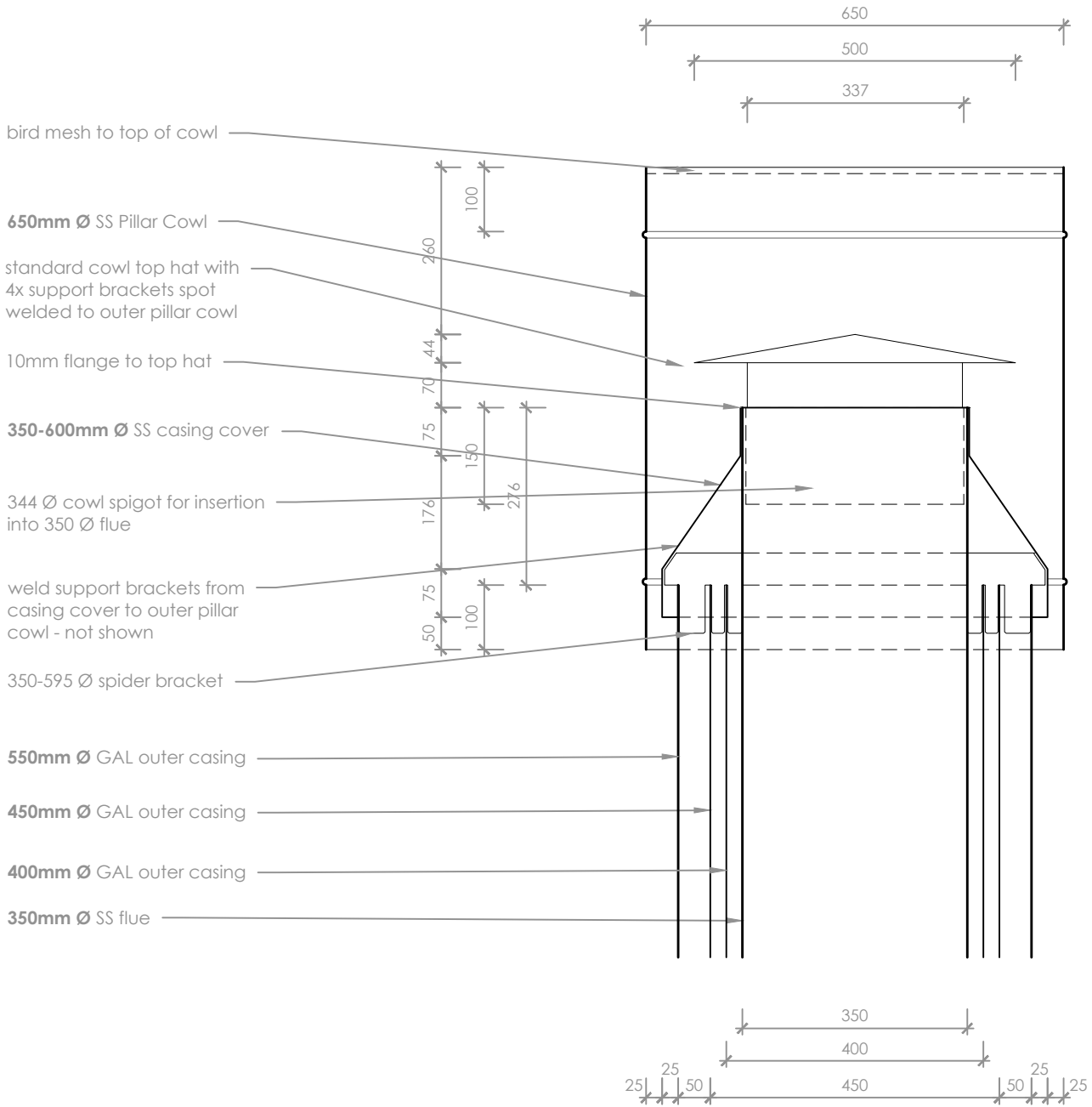
Pillar Cowl Detail
