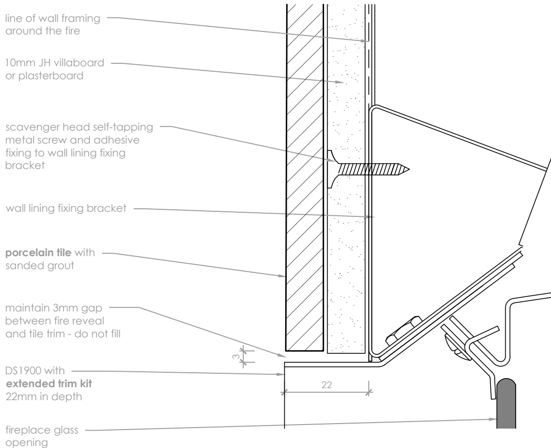
Tile Detail
