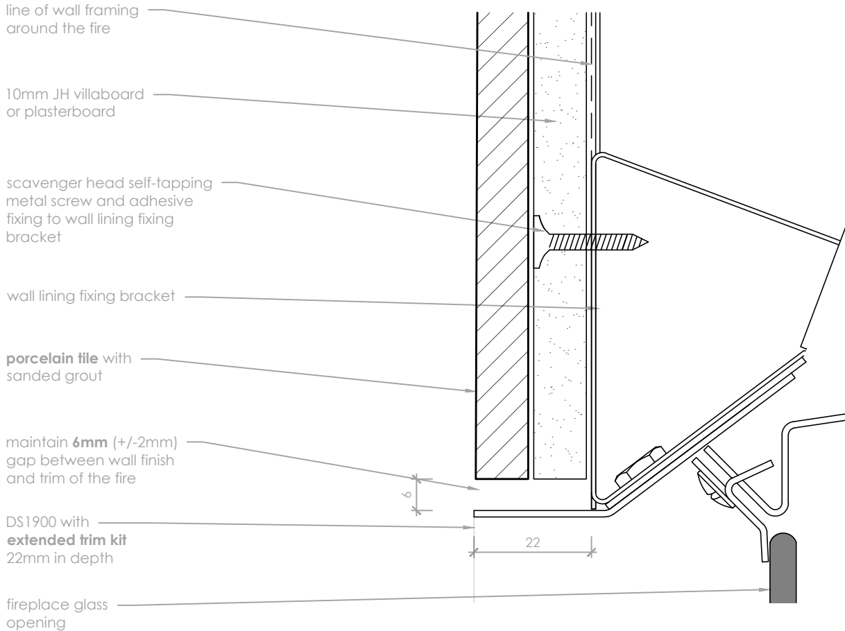
Tile Detail
