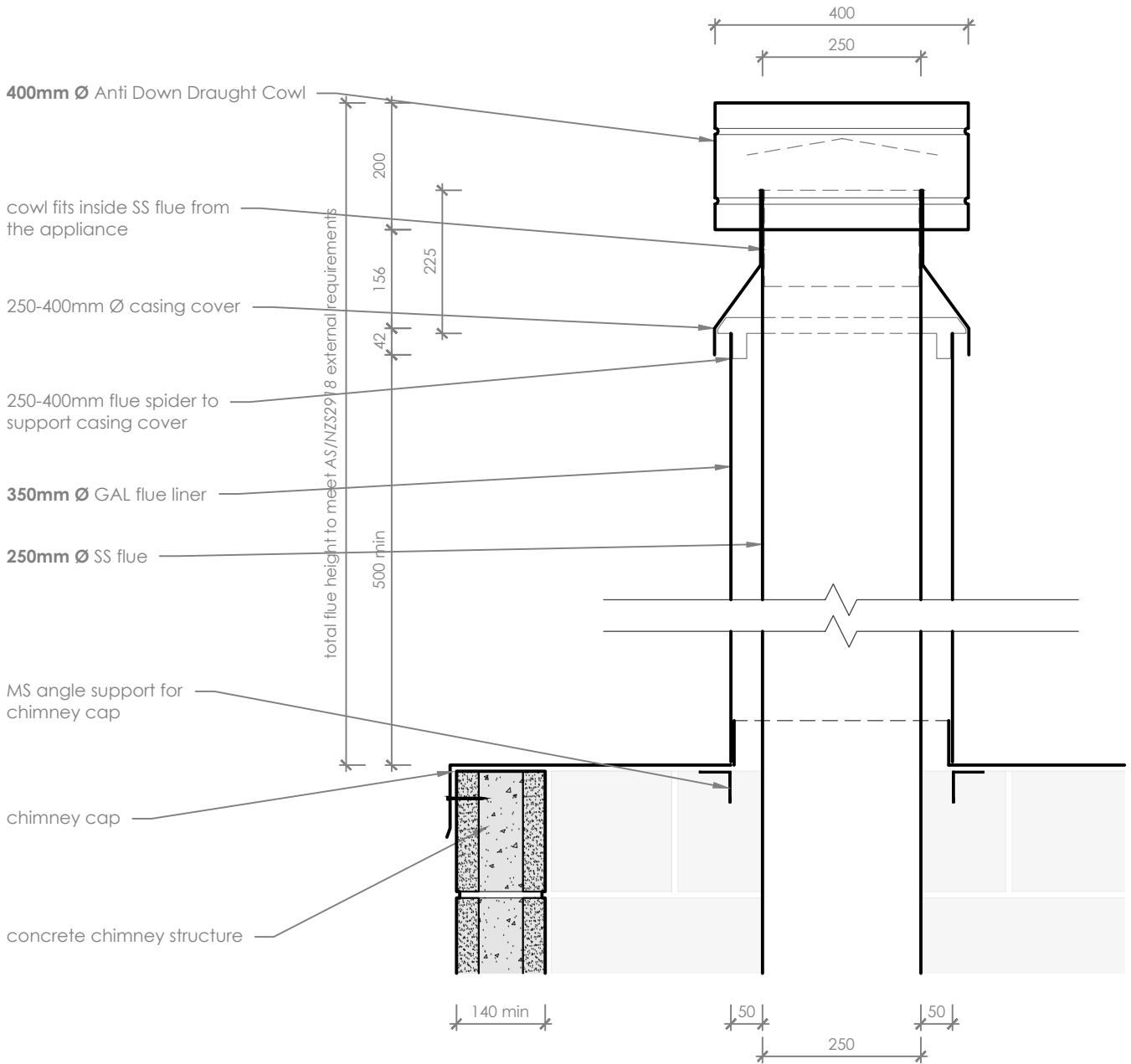
Chimney Cavity Flue Detail 1:10
