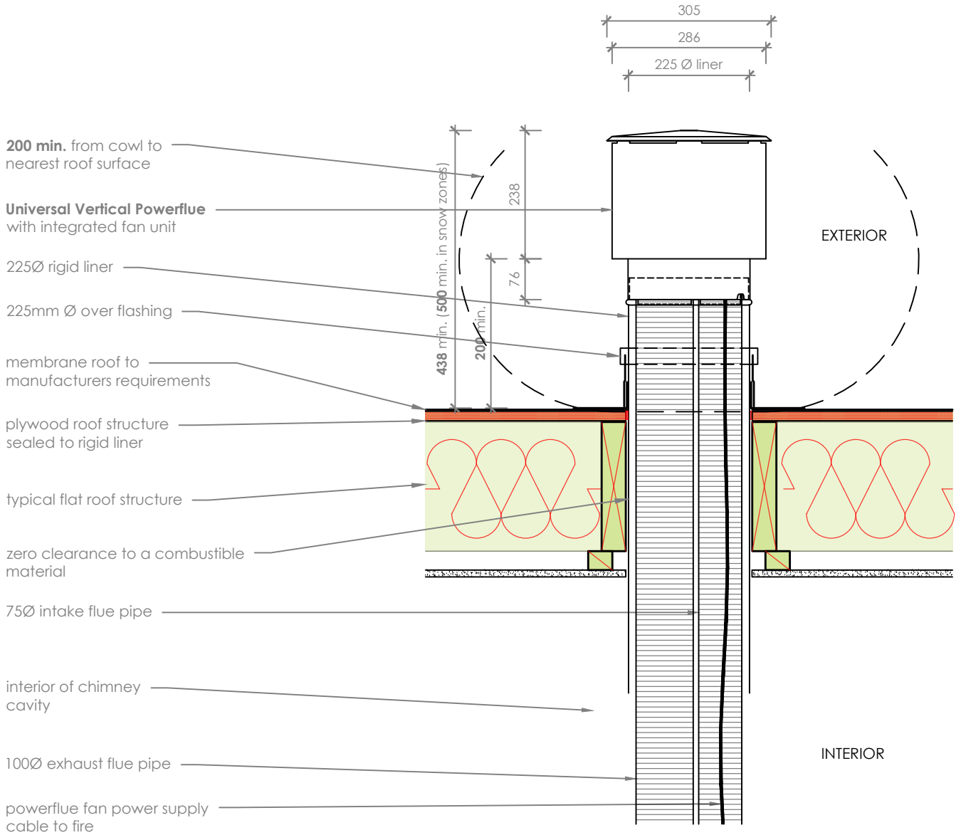
Flue Detail
