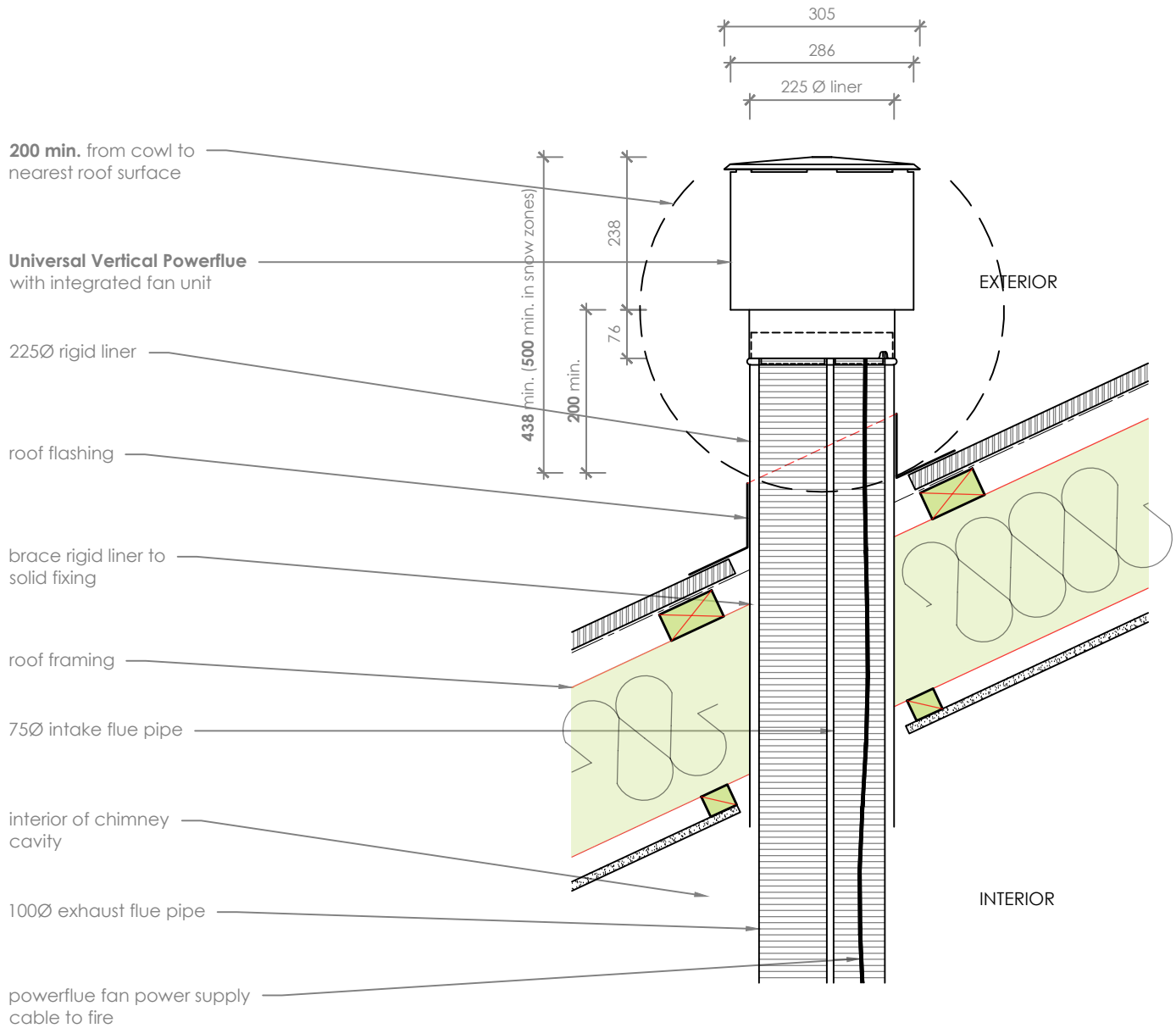
Flue Detail
