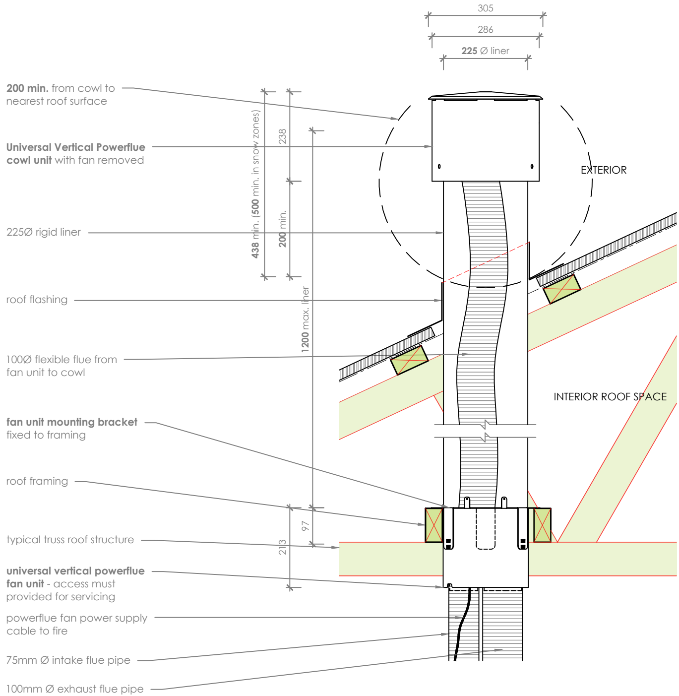
Flue Detail
