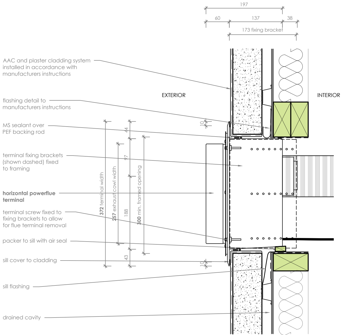
Head/Sill Detail
