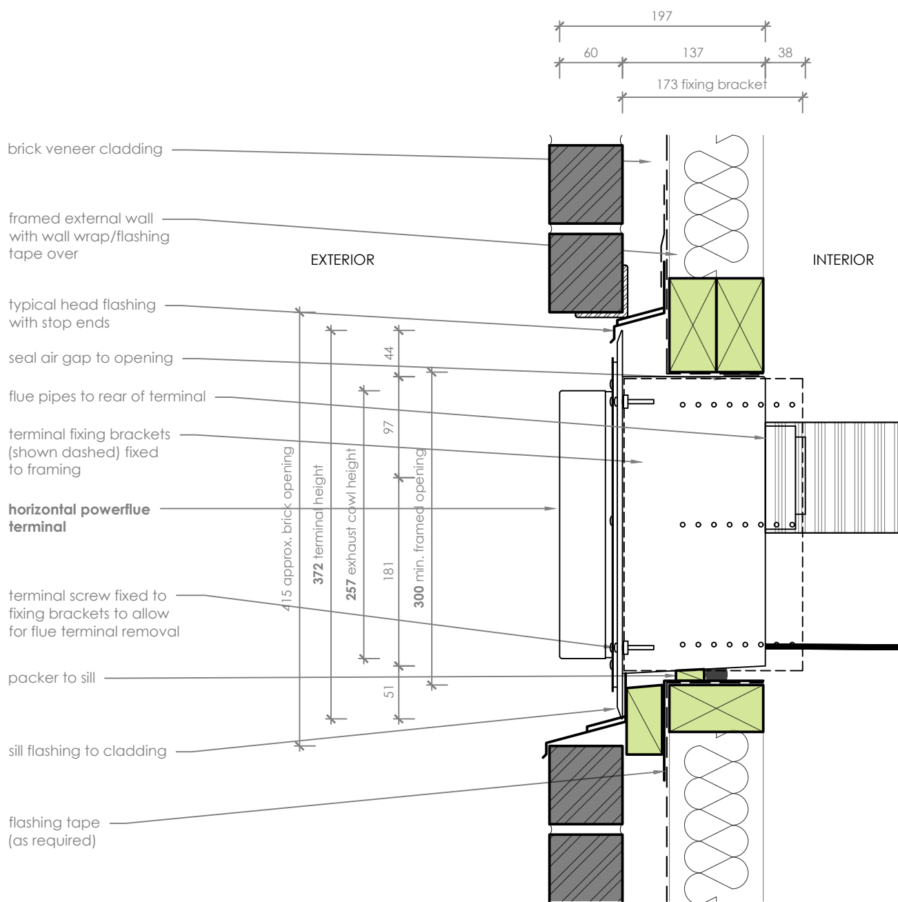
Head/Sill Detail
