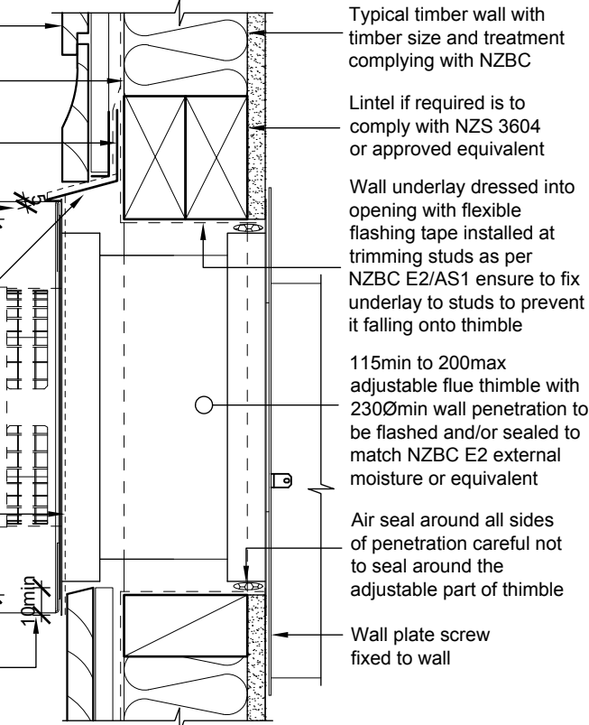
C HEAD AND SILL DETAIL Scale: 1:5
